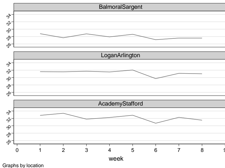
Figure 6-1: Average speed by week at the 50km/h experimental site (Balmoral & Sargent) and control sites in winter
