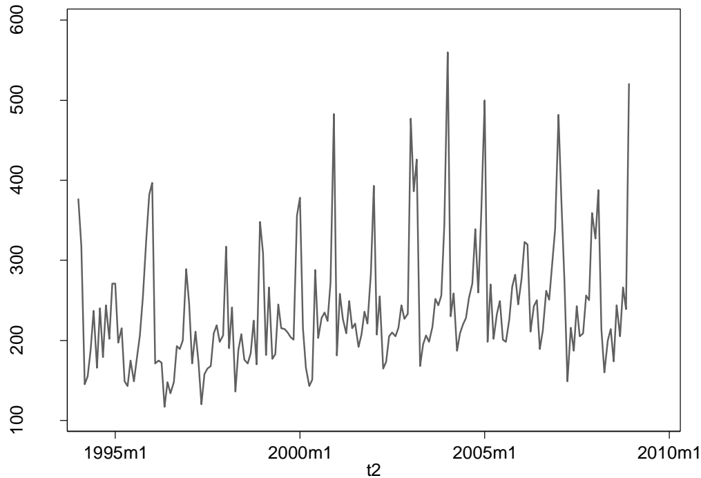
Figure 5-28: Number of rear end crashes in Winnipeg, excluding 48 camera intersections from January 1994 through December 2008
