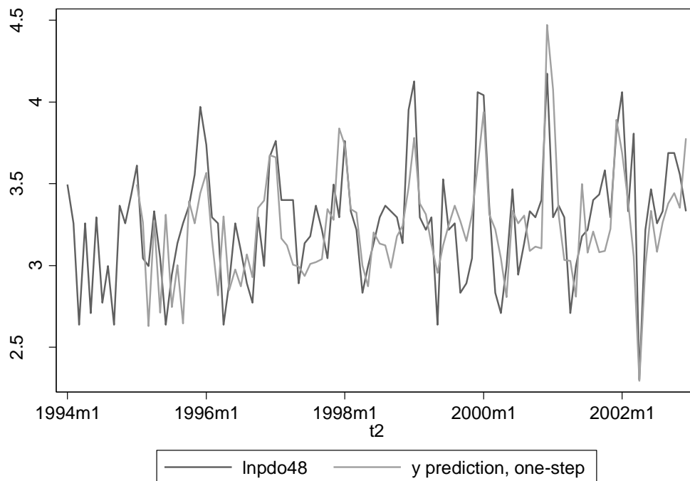
Figure 5-53: log-transformed number of pdo crashes and one-step-ahead predictions according to final model for 48 intersections with cameras, pre-intervention
