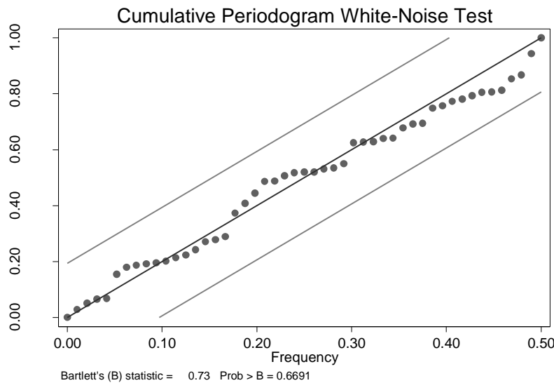
Figure 5-50: Cumulative periodogram white noise test and Bartlett's statistic of the residuals of the final pre-intervention model
