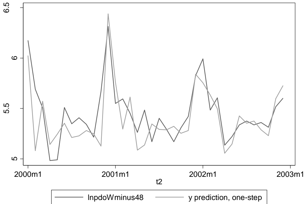
Figure 5-71: log-transformed number of pdo crashes and one-step-ahead predictions according to final model for Winnipeg at intersections without cameras, pre-intervention
