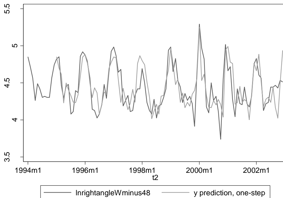
Figure 5-26: log-transformed number of right angle crashes and one-step-ahead predictions according to final model for Winnipeg excluding 48 camera intersections, pre-intervention
