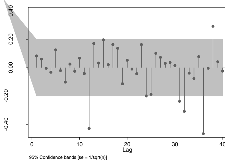
Figure 5-31: Partial autocorrelation of pre-intervention log-transformed, seasonally differenced rear end crash series in Winnipeg, excluding 48 camera intersections
