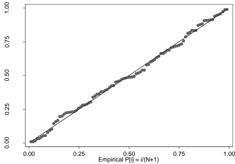
Figure 5-16: Normal density plot of the residuals of the final pre-intervention model
