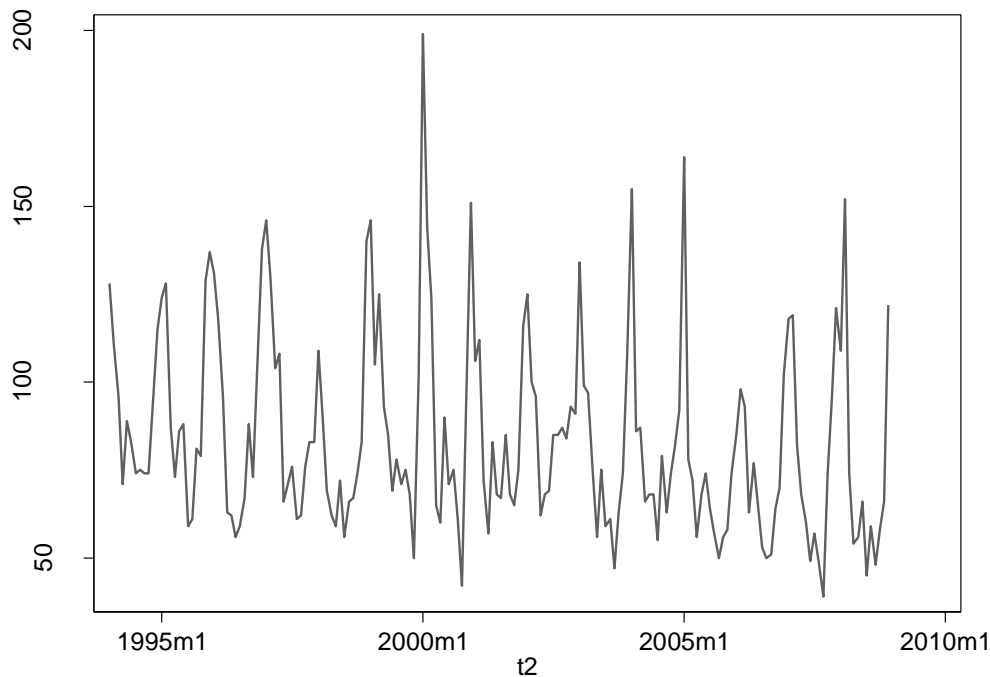
Figure 5-19: Number of right angle crashes in Winnipeg, excluding 48 camera intersections from January 1994 through December 2008
