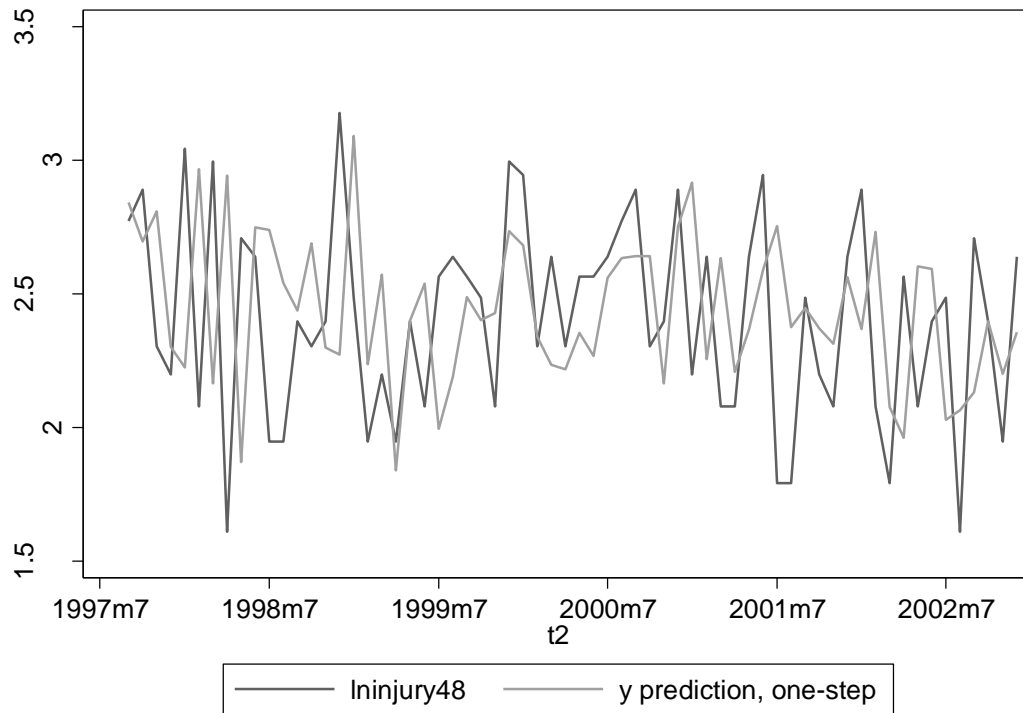
Figure 5-44: log-transformed number of injury crashes and one-step-ahead predictions according to final model for 48 intersections with cameras, pre-intervention
