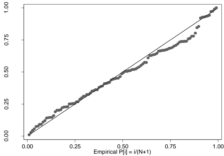
Figure 5-6: Standardized normal probability plot of the residuals of the final pre-intervention model
