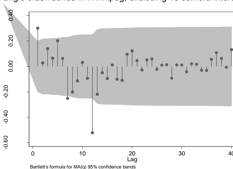
Figure 5-21: Autocorrelation of pre-intervention log-transformed, seasonally differenced right angle crash series in Winnipeg, excluding 48 camera intersections
