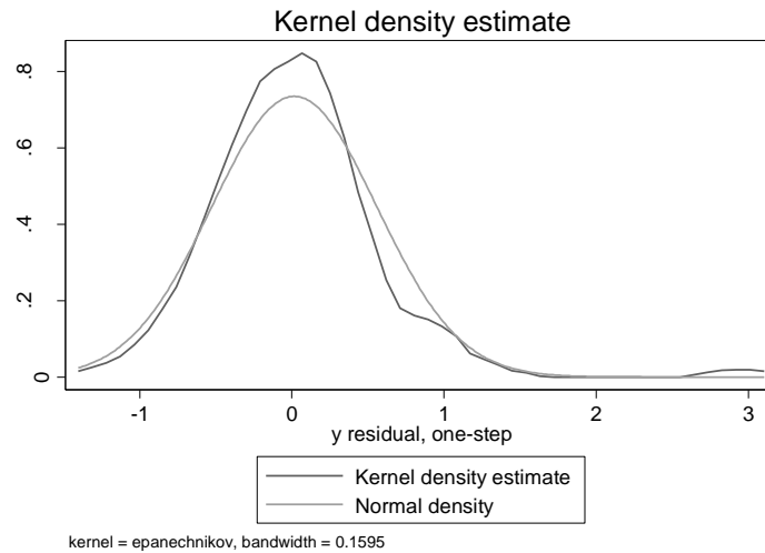
Figure 5-7: Normal density plot of the residuals of the final pre-intervention model
