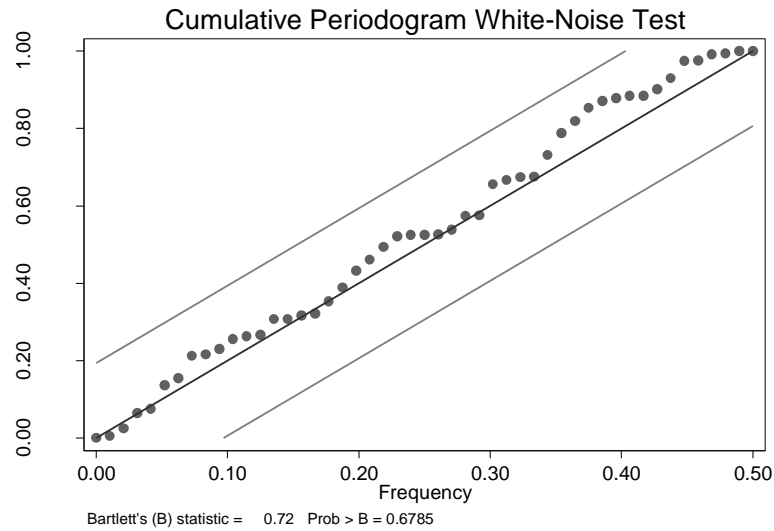
Figure 5-23: Cumulative periodogram white noise test and Bartlett's statistic of the residuals of the final pre-intervention model
