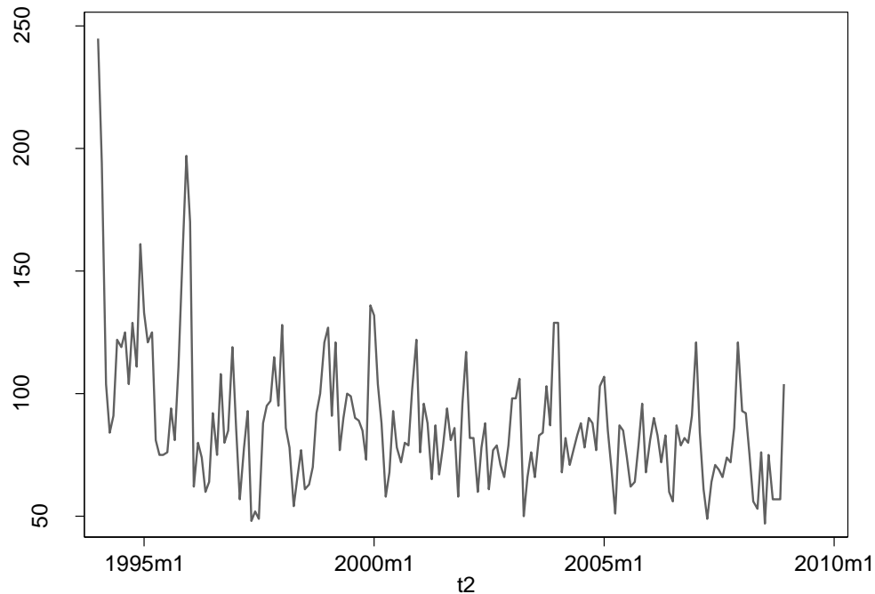
Figure 5-55: Number of injury crashes in Winnipeg at intersections without cameras from January 1994 through December 2008
