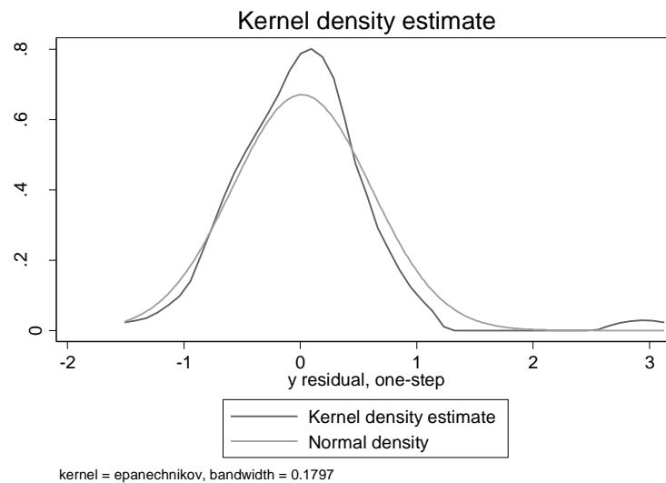
Figure 5-43: Normal density plot of the residuals of the final pre intervention model
