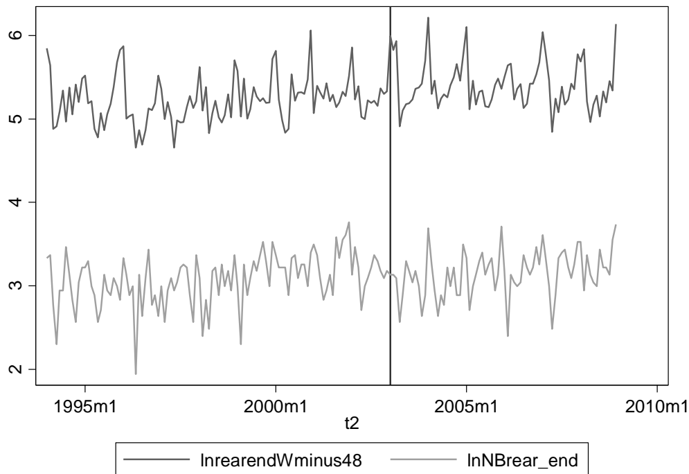
Figure 5-36: log-transformed number of rear end crashes in the experimental group (Winnipeg, \ln \text{rearendWminus48} ) and the control group (New Brunswick, \ln \text{NBrear\_end} )
