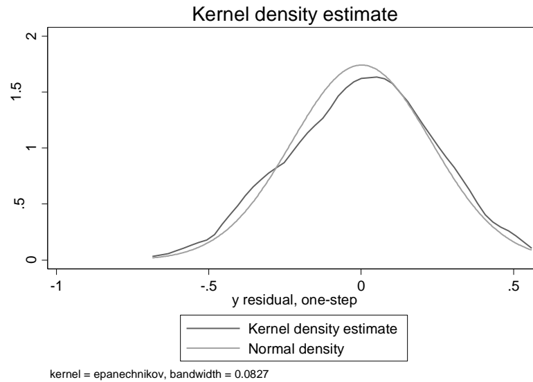
Figure 5-34: Normal density plot of the residuals of the final pre-intervention model
