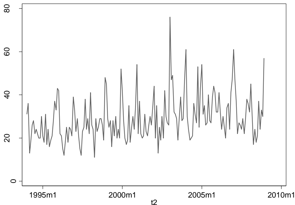
Figure 5-10: Number of rear end crashes in Winnipeg at 48 intersections with cameras from January 1994 through December 2008
