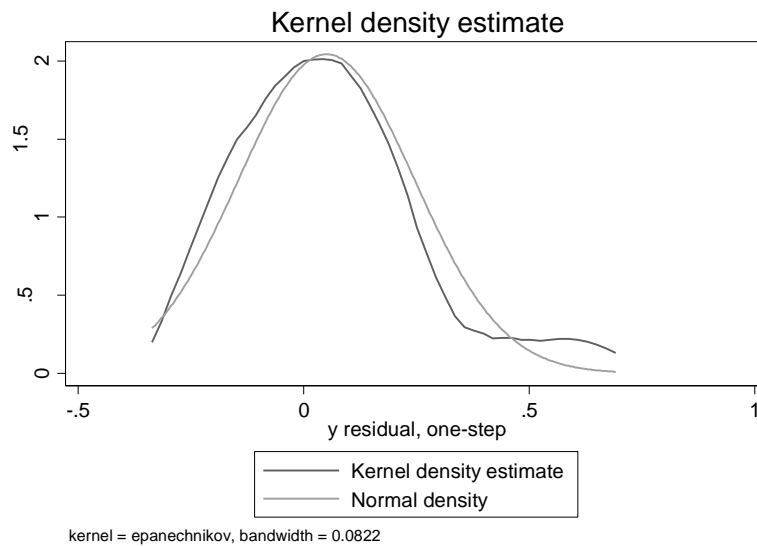
Figure 5-70: Normal density plot of the residuals of the final pre-intervention model
