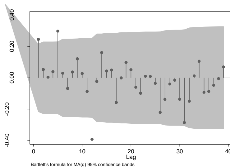
Figure 5-57: Autocorrelation of pre-intervention log-transformed, seasonally differenced injury crashes in Winnipeg at intersections without cameras
