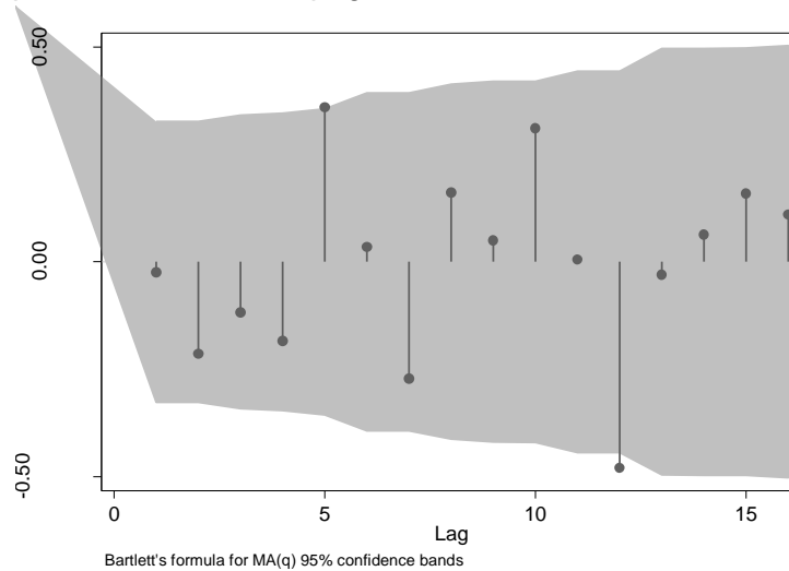
Figure 5-66: Autocorrelation of pre-intervention log-transformed, seasonally differenced pdo crashes in Winnipeg at intersections without cameras
