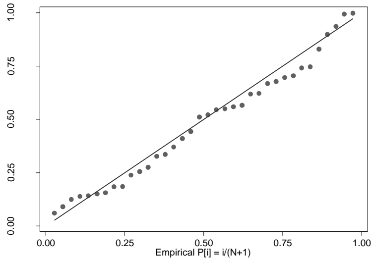
Figure 5-69: Standardized normal probability plot of the residuals of the final pre-intervention model
