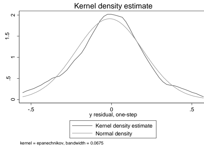
Figure 5-25: Normal density plot of the residuals of the final pre-intervention model
