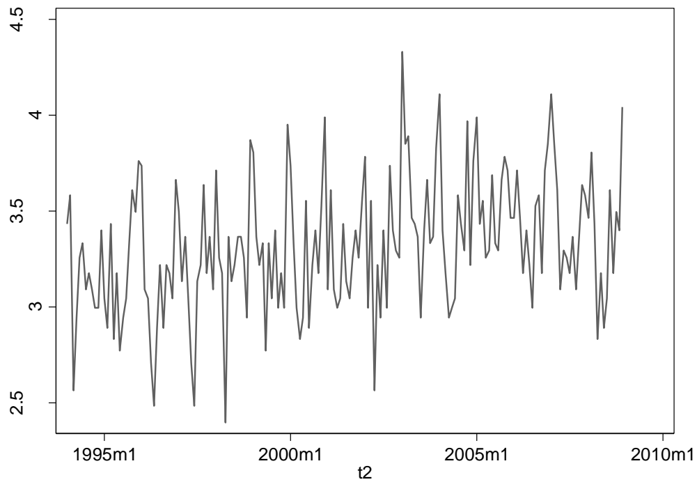
Figure 5-11: Log of the number of rear end crashes in Winnipeg at 48 intersections with cameras from January 1994 through December 2008
