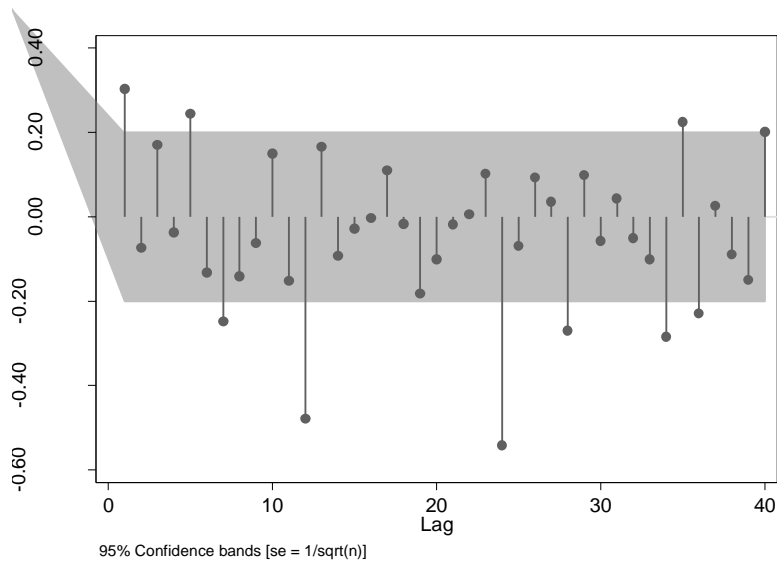
Figure 5-22: Partial autocorrelation of pre-intervention log-transformed, seasonally differenced right angle crash series in Winnipeg, excluding 48 camera intersections
