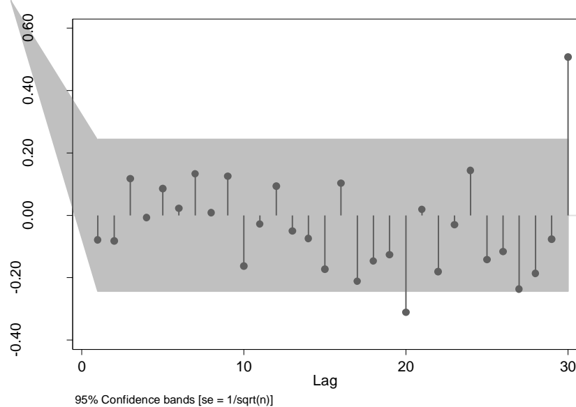
Figure 5-40: Partial autocorrelation of pre-intervention log-transformed injury crashes
