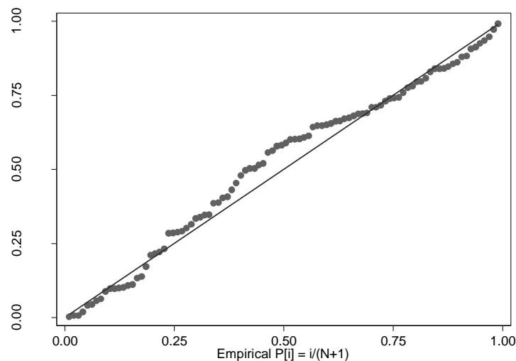
Figure 5-51: Standardized normal probability plot of the residuals of the final pre-intervention model
