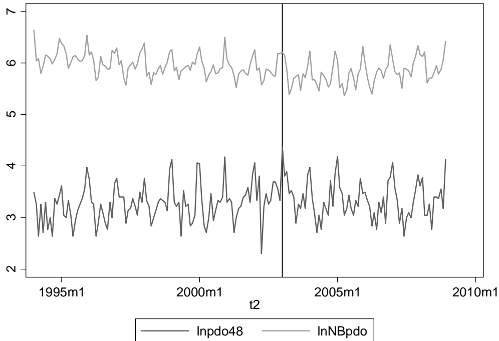
Figure 5-54: log-transformed number of pdo crashes in the experimental group (Winnipeg, \ln pdo48 ) and the control group (New Brunswick, \ln NB pdo )
