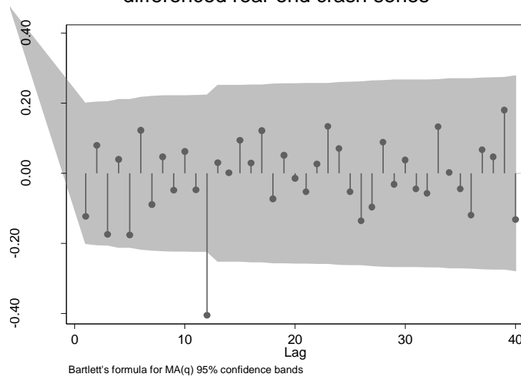
Figure 5-12: Autocorrelation of the pre-intervention log-transformed and seasonally differenced rear end crash series
