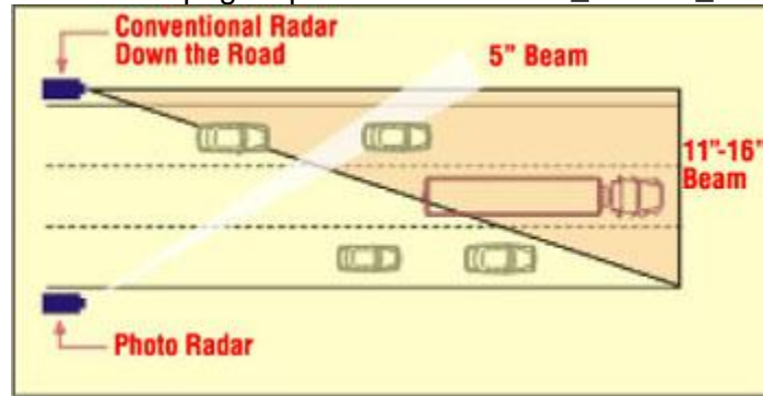
Figure 3-1: Difference in beam coverage between conventional radar and photo radar ( http://www.winnipeg.ca/police/safeststreets/is_camera_tech.stm )
