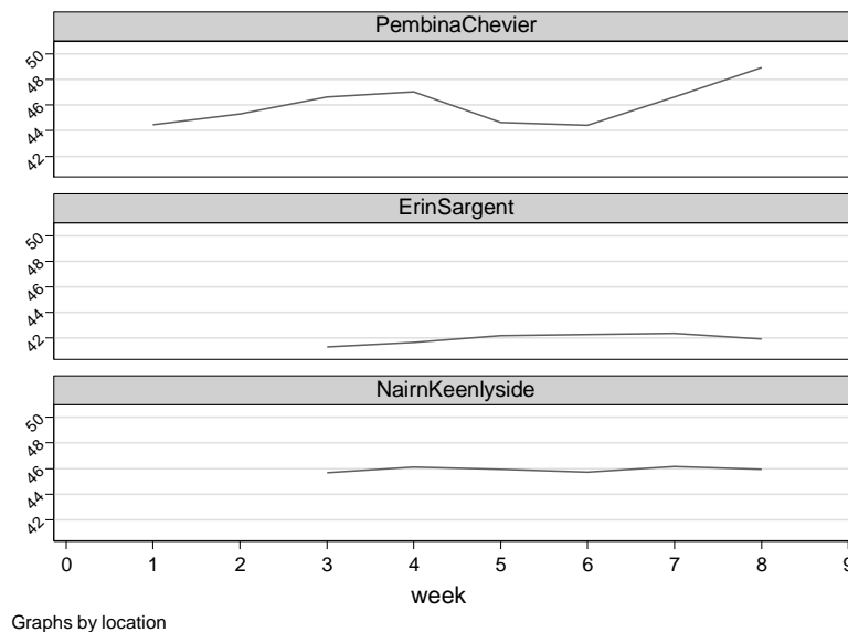
Figure 6-2: Average speed by week at the 60km/h experimental site (Pembina & Chevier) and control sites in winter
