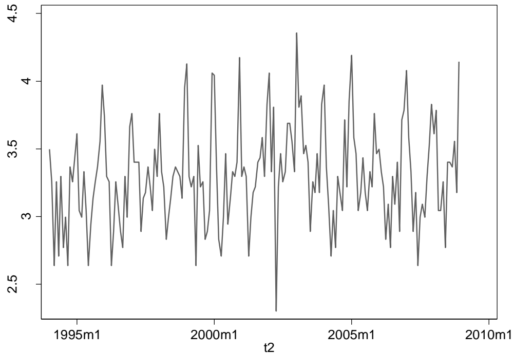
Figure 5-47: Log of the number of pdo crashes in Winnipeg at 48 intersections with cameras from January 1994 through December 2008
