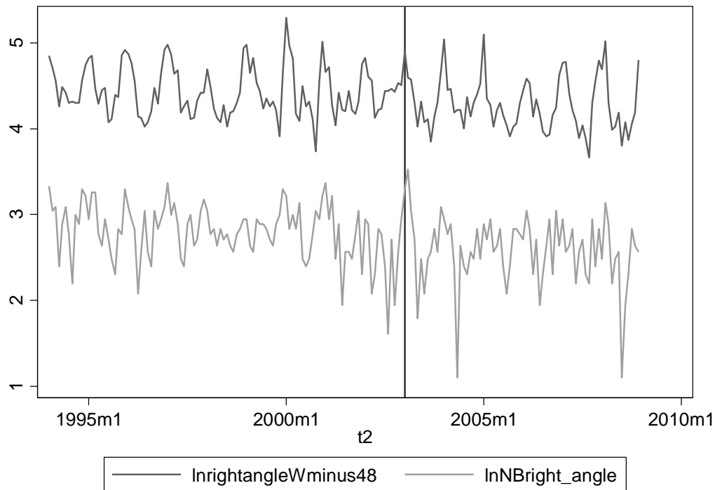
Figure 5-27: log-transformed number of right angle crashes in the experimental group (Winnipeg, \ln\text{rightangleWminus48} ) and the control group (New Brunswick, \ln\text{NBright\_angle} )
