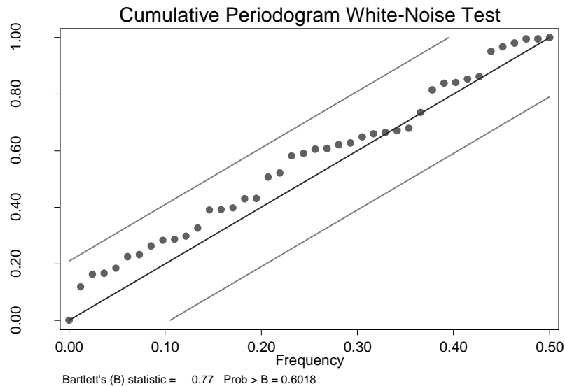
Figure 5-59: Cumulative periodogram white noise test and Bartlett's statistic of the residuals of the final pre-intervention model
