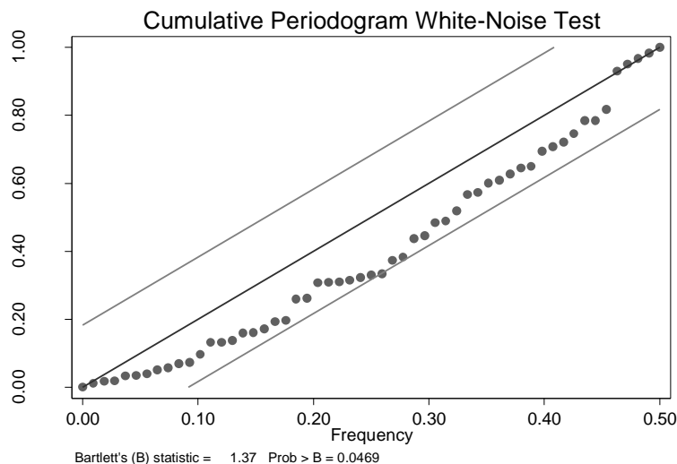
Figure 5-5: Cumulative periodogram white noise test and Bartlett's statistic of the residuals of the final pre-intervention model
