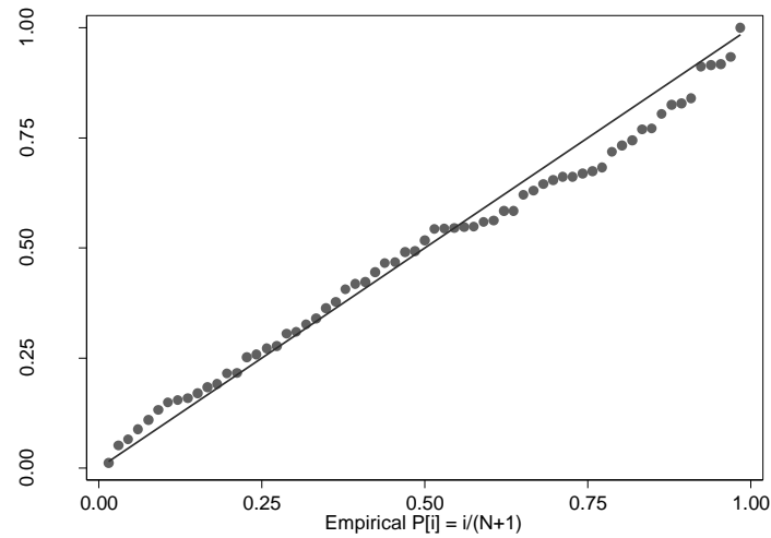
Figure 5-42: Standardized normal probability plot of the residuals of the final pre intervention model
