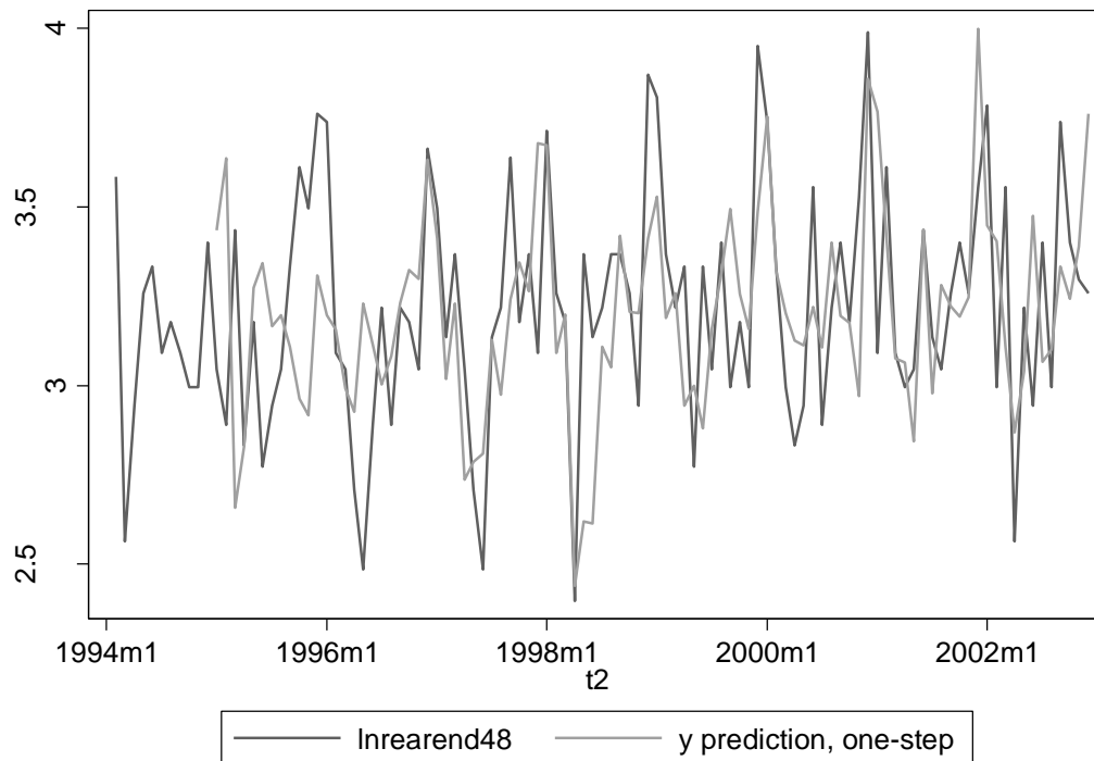
Figure 5-17: log-transformed number of rear end crashes and one-step-ahead predictions according to final model for 48 intersections with cameras, pre-intervention
