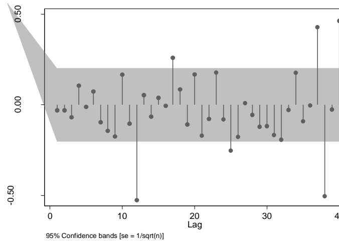
Figure 5-49: Partial autocorrelation of pre-intervention log-transformed, seasonally differenced pdo crashes
