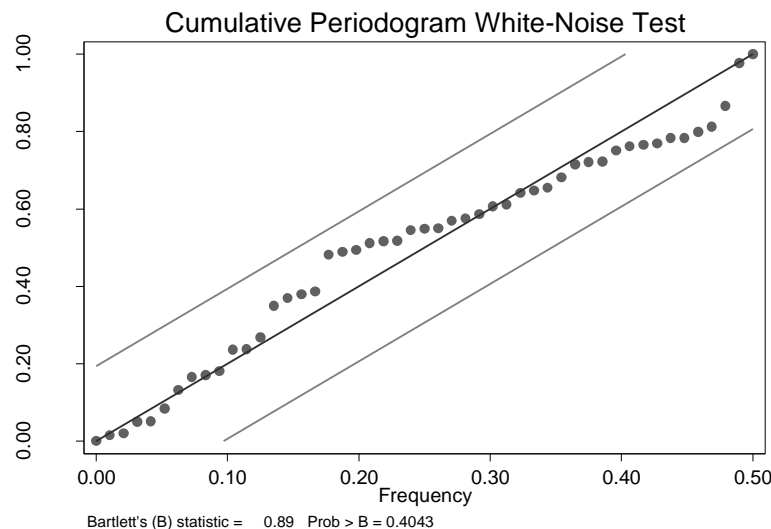
Figure 5-14: Cumulative periodogram white noise test and Bartlett's statistic of the residuals of the final pre-intervention model
