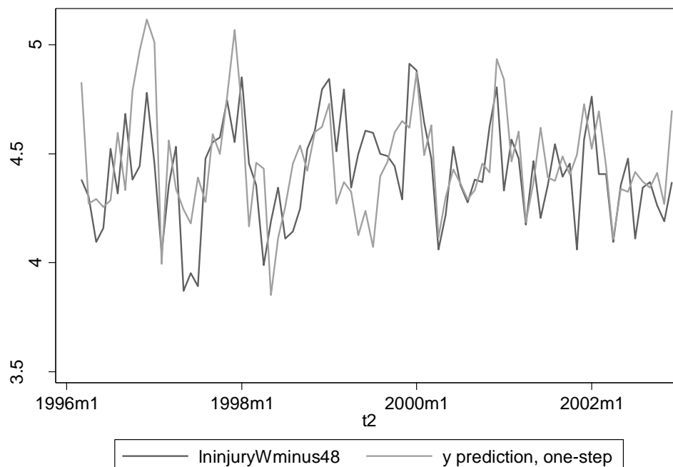
Figure 5-62: log-transformed number of injury crashes and one-step-ahead predictions according to final model for Winnipeg at intersections without cameras, pre-intervention
