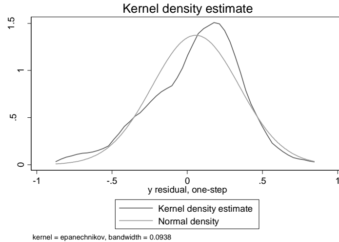
Figure 5-52: Normal density plot of the residuals of the final pre-intervention model
