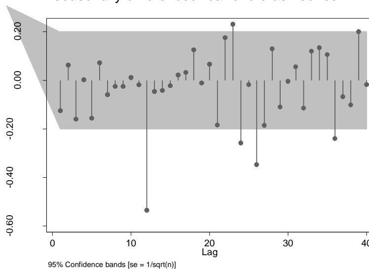
Figure 5-13: Partial autocorrelation of the pre-intervention log-transformed and seasonally differenced rear end crash series
