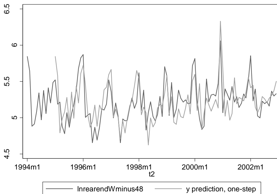
Figure 5-35: log-transformed number of rear end crashes and one-step-ahead predictions according to final model for Winnipeg, excluding 48 camera intersections, pre-intervention
