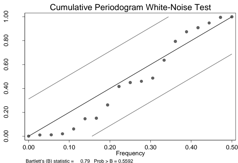
Figure 5-68: Cumulative periodogram white noise test and Bartlett's statistic of the residuals of the final pre-intervention model
