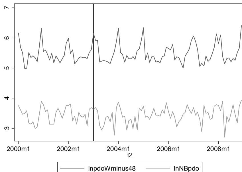
Figure 5-72: log-transformed number of pdo crashes in the experimental group (Winnipeg, ln pdoWminus48) and the control group (New Brunswick, lnNBpdo)
