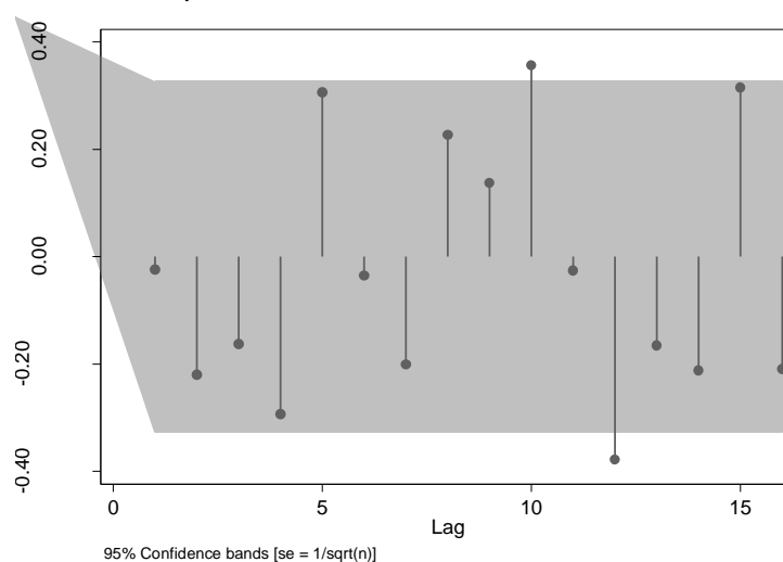
Figure 5-67: Partial autocorrelation of pre-intervention log-transformed, seasonally differenced pdo crashes at intersections without cameras
