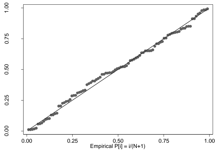
Figure 5-24: Standardized normal probability plot of the residuals of the final pre-intervention model
