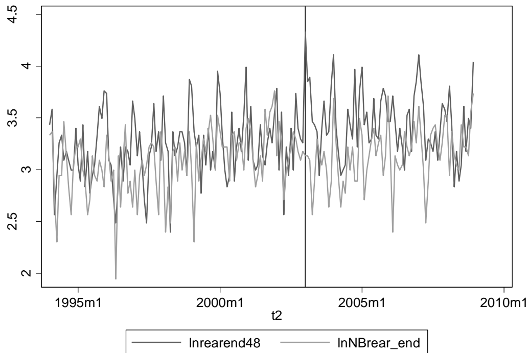
Figure 5-18: log-transformed number of rear end crashes in the experimental group (Winnipeg, lnrearend48) and the control group (New Brunswick, lnNBrear_end)
