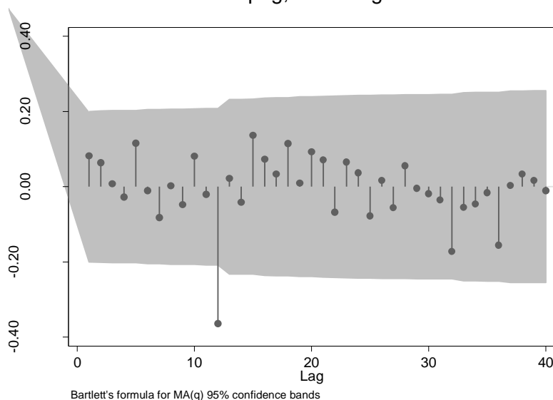
Figure 5-30: Autocorrelation of pre-intervention log-transformed, seasonally differenced rear end crash series in Winnipeg, excluding 48 camera intersections
