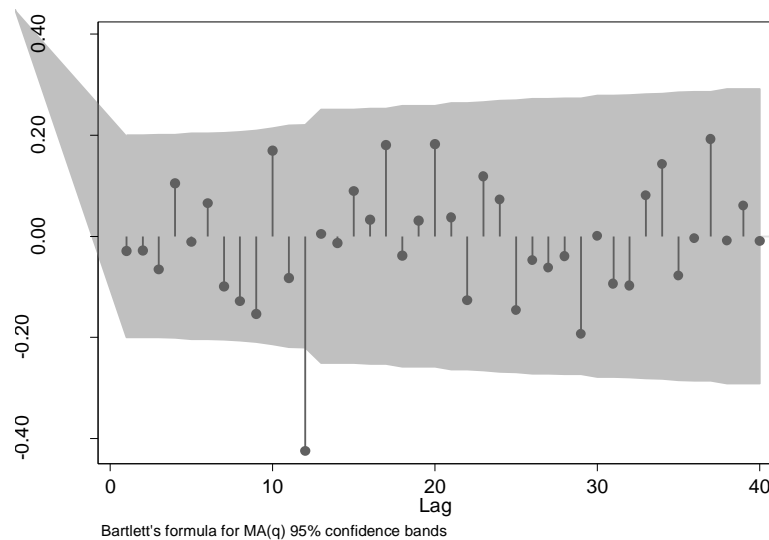
Figure 5-48: Autocorrelation of pre-intervention log-transformed, seasonally differenced pdo crashes
