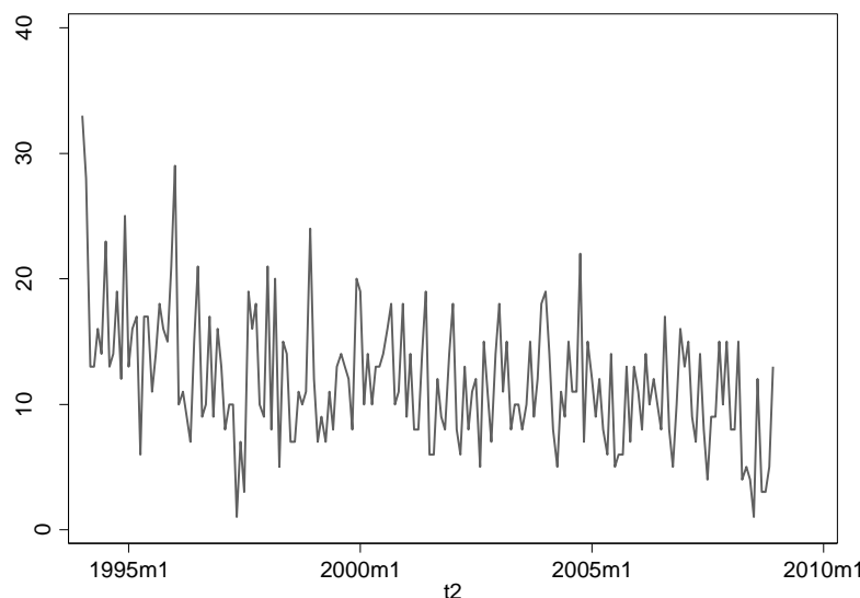
Figure 5-37: Number of injury crashes in Winnipeg at 48 intersections with cameras from January 1994 through December 2008
