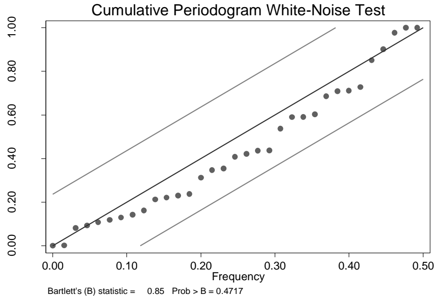
Figure 5-41: Cumulative periodogram white noise test and Bartlett's statistic of the residuals of the final pre intervention model
