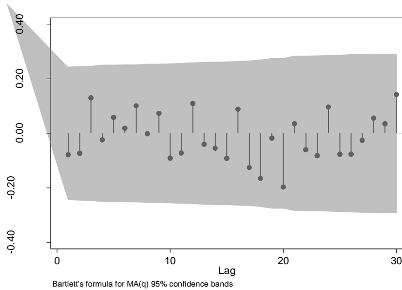
Figure 5-39: Autocorrelation of pre-intervention log-transformed injury crashes
