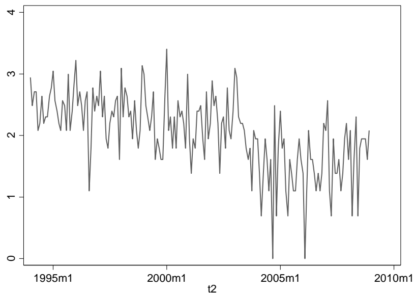
Figure 5-2: Log of the number of right angle crashes in Winnipeg at 48 intersections with cameras from January 1994 through December 2008
