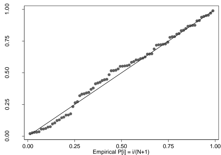
Figure 5-60: Standardized normal probability plot of the residuals of the final pre-intervention model
