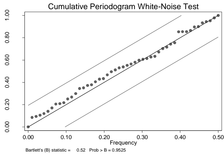
Figure 5-32: Cumulative periodogram white noise test and Bartlett's statistic of the residuals of the final pre-intervention model
